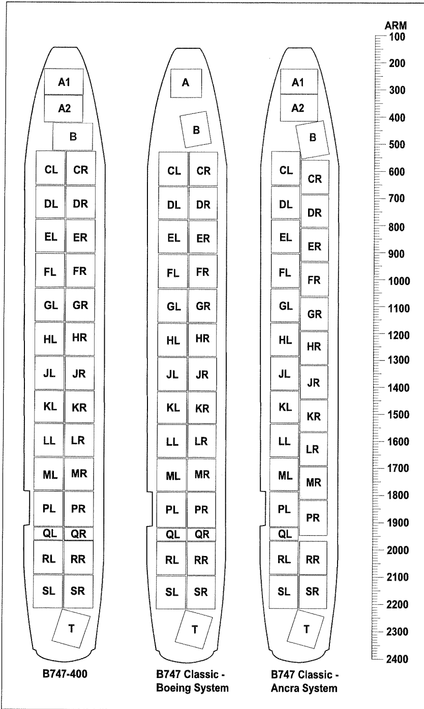
Figure 33.1.17 All B747 Main Deck Configurations
